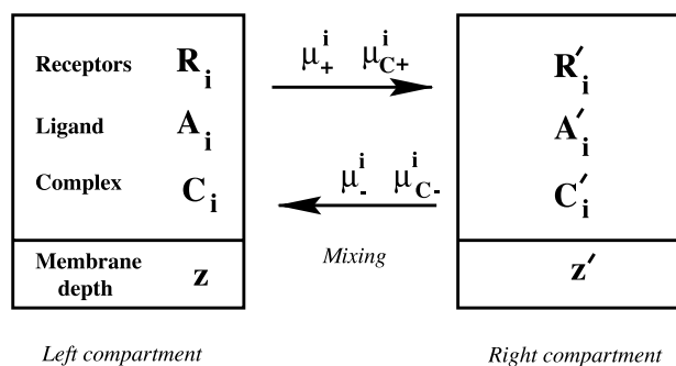
FIGURE 10 Schematic two-component model for study of amplification by membrane depth variation. Mixing rates for R_i and A_i are \mu_{\pm}^i ; those of C_i are \mu_{C\pm}^i .
